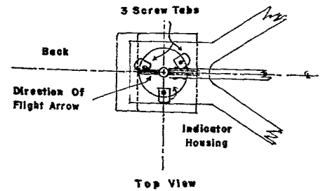
Screw Tab Arrangement Sketch No 2
