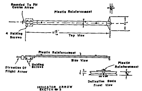
INDICATOR ARROW SKETCH No 3
